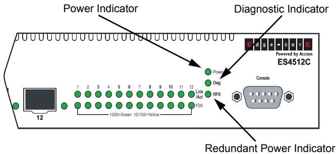
Figure 1-7. ES4512C System LEDs
