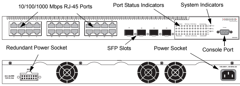
Figure 1-2. ES4524C Front and Rear Panels
