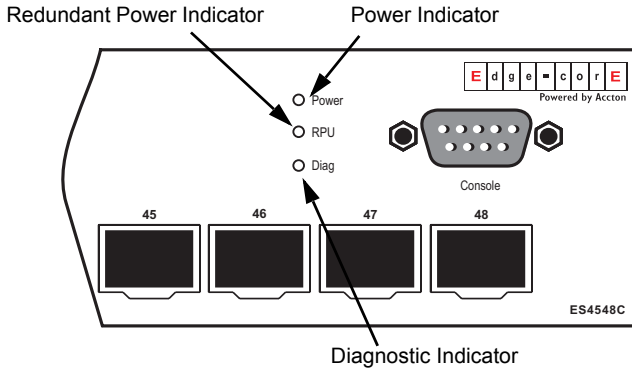
Figure 1-9. ES4548C System LEDs
