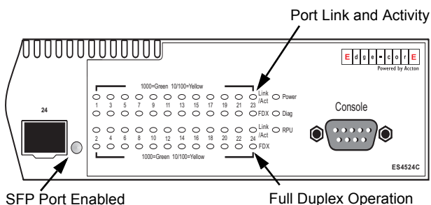
Figure 1-5. ES4524C Port LEDs
