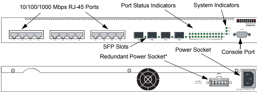
Figure 1-1. ES4512C Front and Rear Panels
